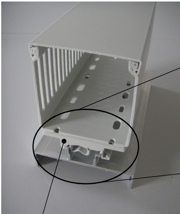
snap-in clip Rastclip
